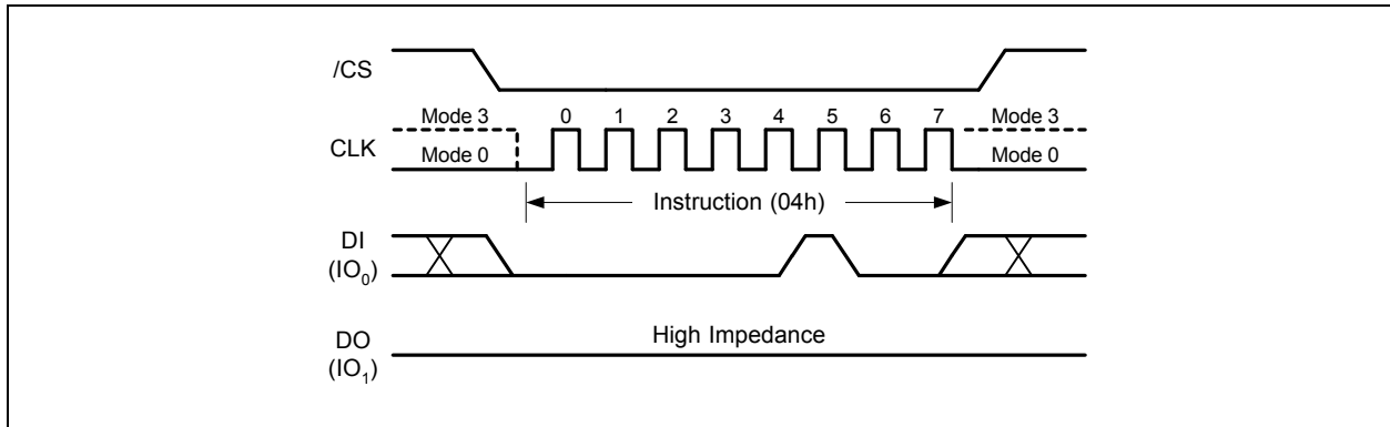
Figure 7. Write Disable Instruction
