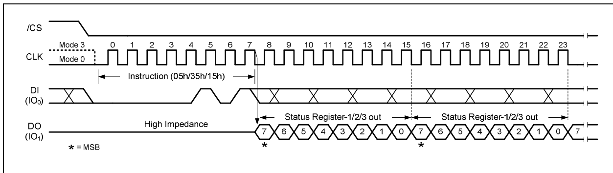
Figure 8. Read Status Register Instruction
