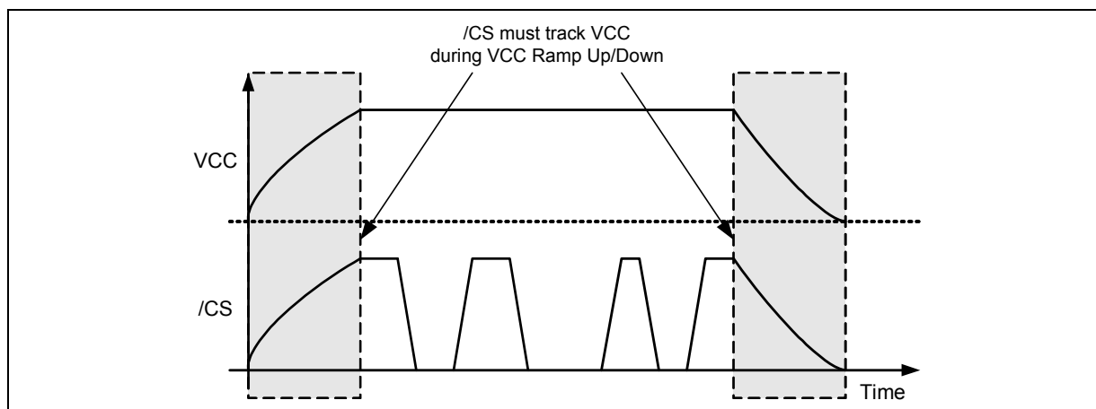
Figure 54b. Power-up, Power-Down Requirement
